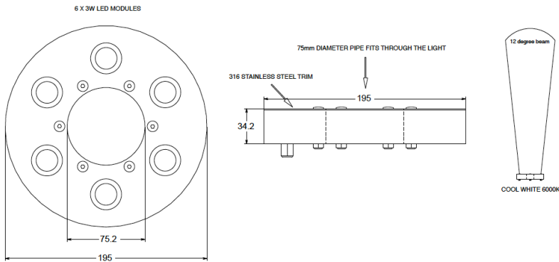
18W, 12V, DC LED RING LIGHT
